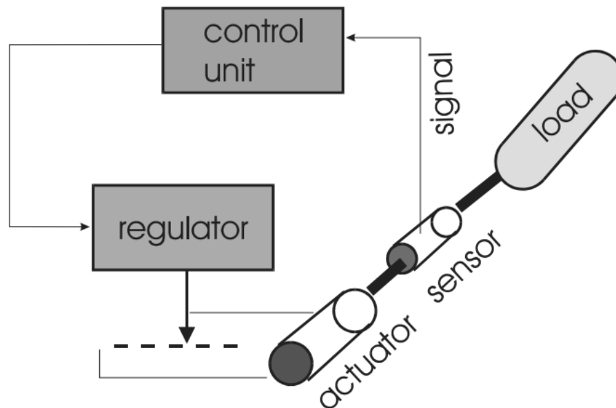
Fig.2 A mechatronic design for a manipulator actuator
